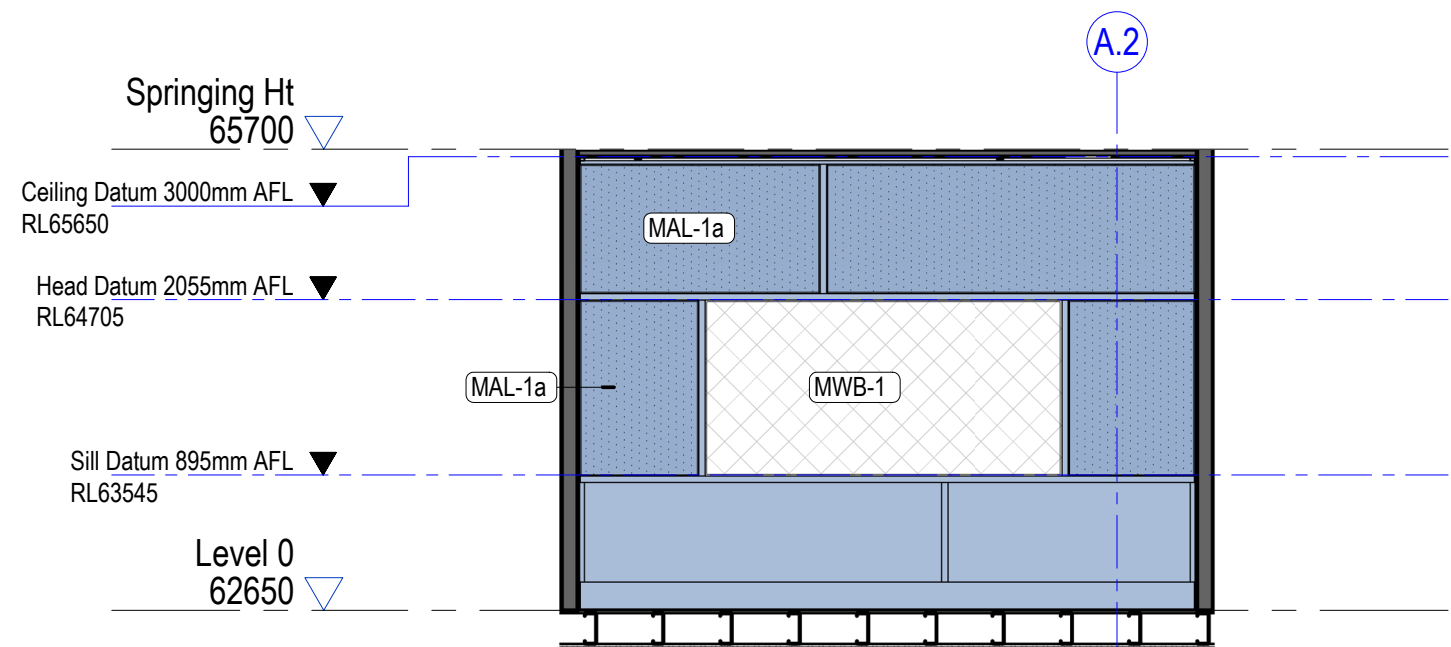
4 0.27 - Meeting 5 - South Elevation 1 : 50
