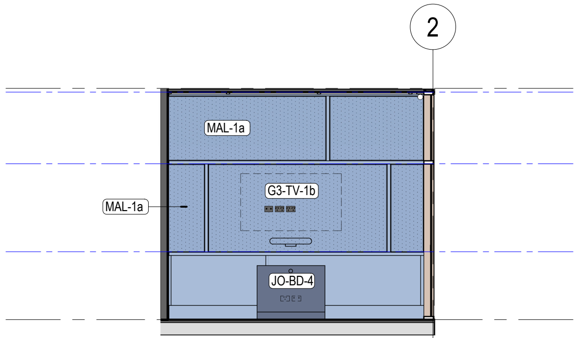
5 0.27 - Meeting 5 - West Elevation 1 : 50
