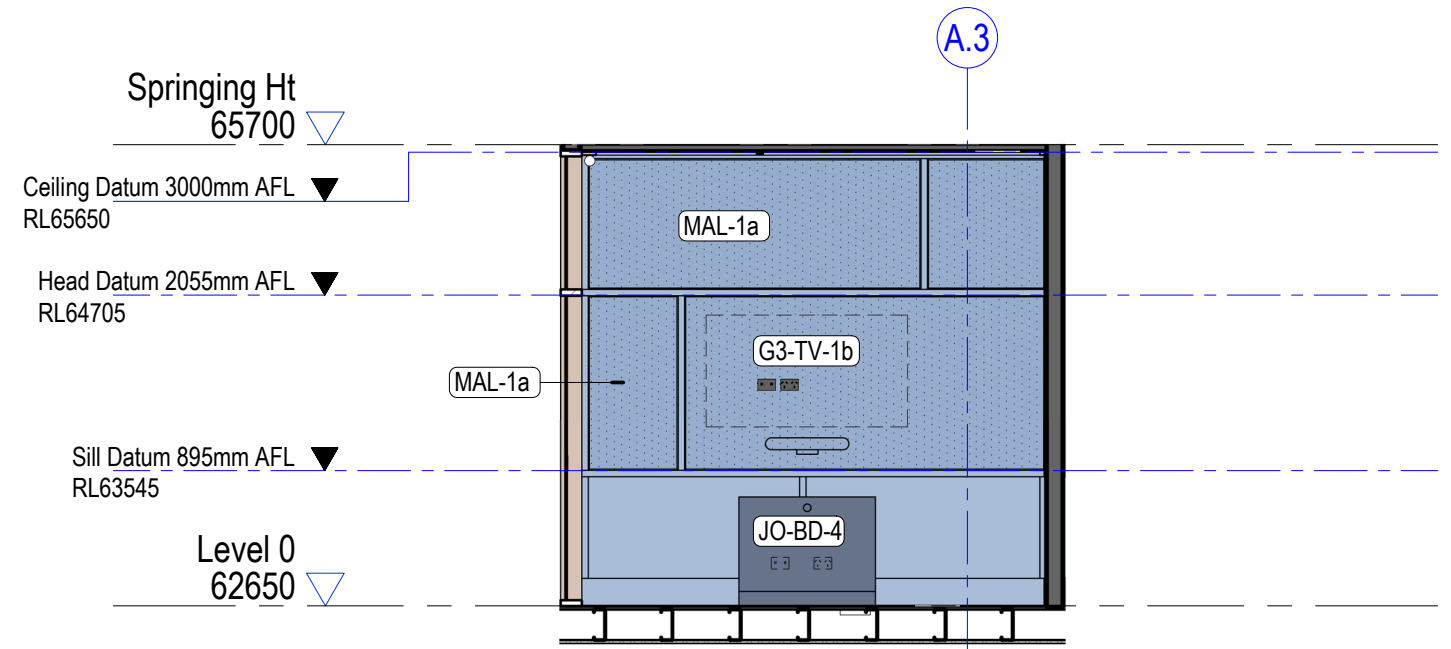
9 0.28 - Meeting 6 - South Elevation 1 : 50
