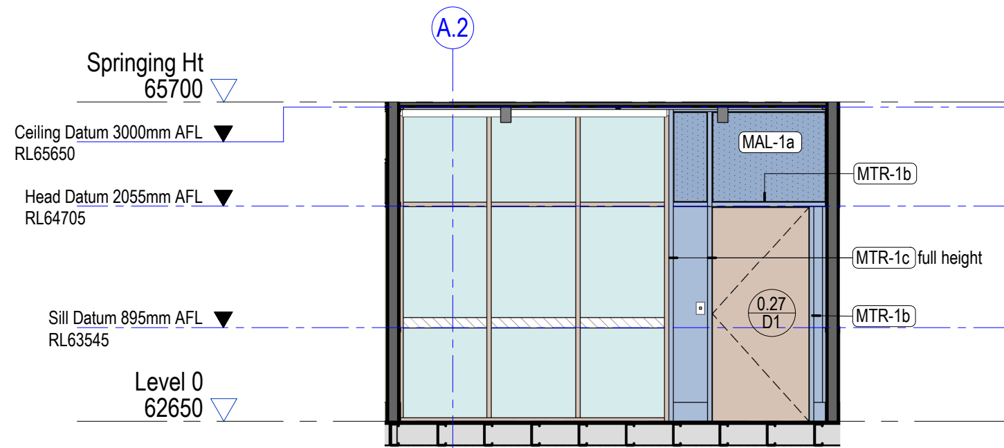
2 0.27 - Meeting 5 - North Elevation 1 : 50
